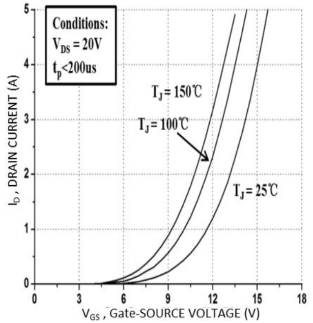
Fig.2 Output Characteristics
