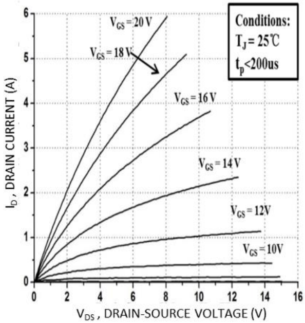
Fig.1 Output Characteristics
