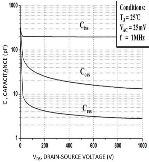
Fig.5 Capacitance
